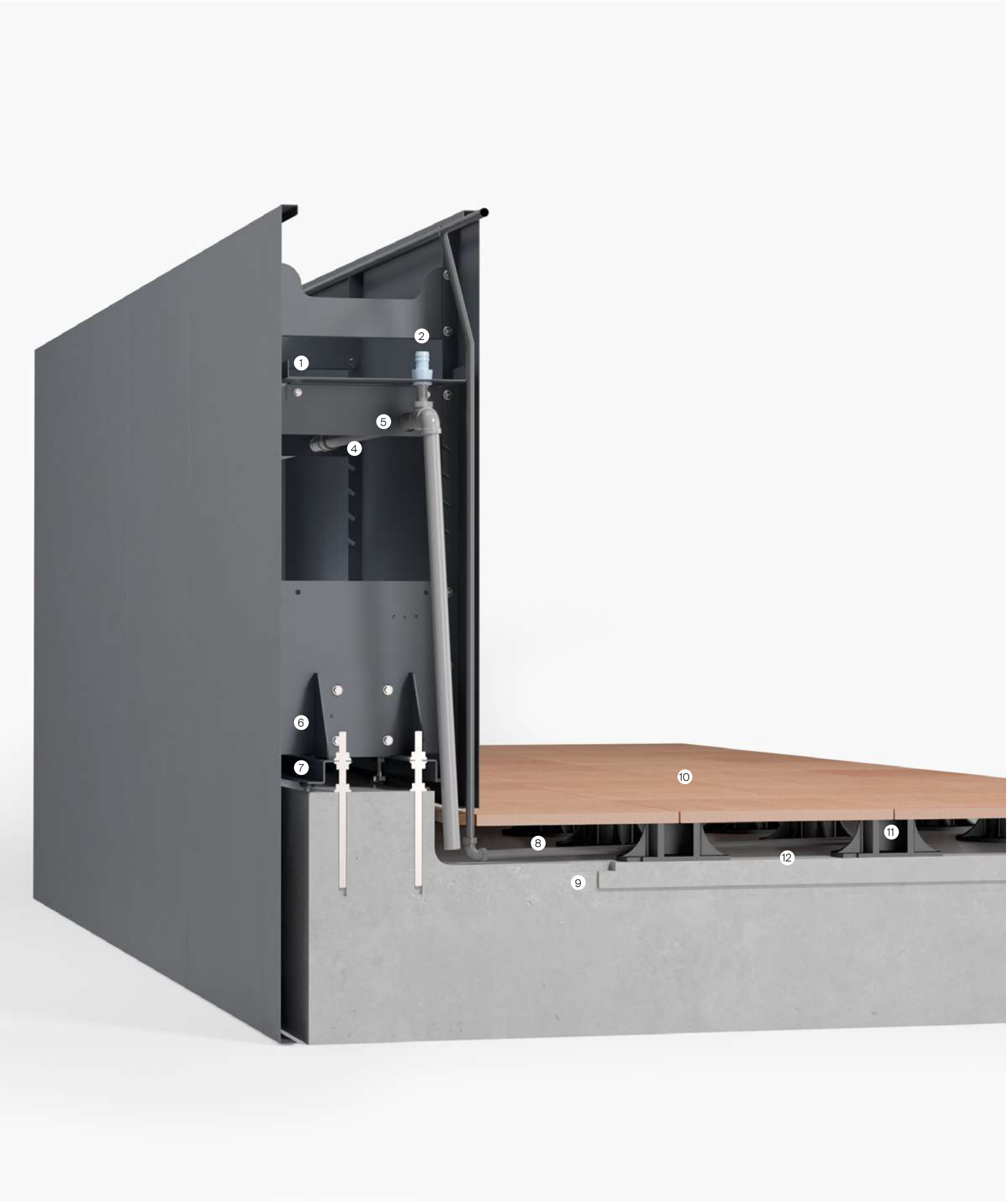
1 Height-adjusted base 2 Standard overflow drain 3 Drip line connected to the irrigation pipe 4 Water channelling pipe with T fittings for overflow discharge insertion
