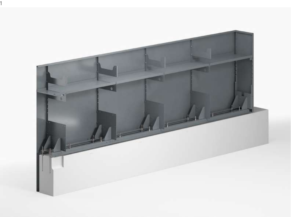
1 Modularte patented "tracks" mounting system 2 Bracket plate and stiffening wall
